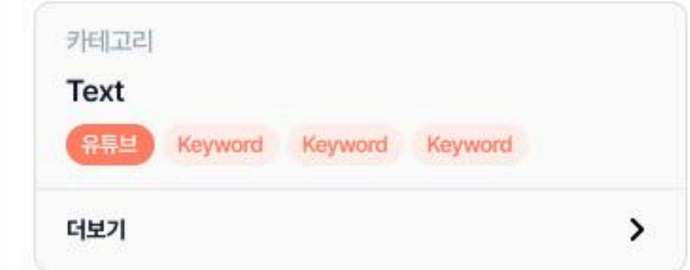
Content Card
