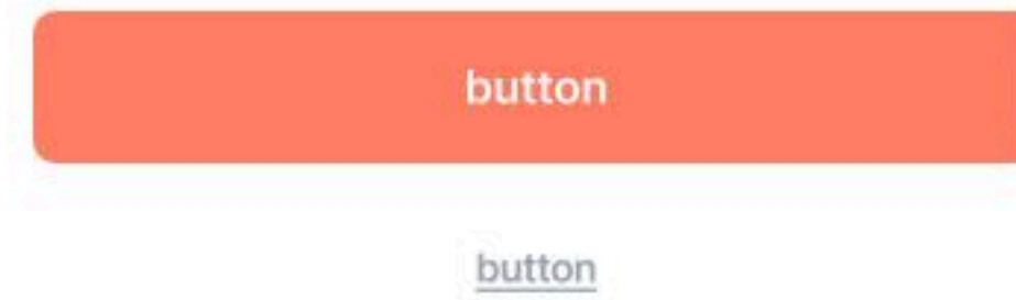
Button
