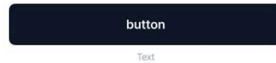
Button
