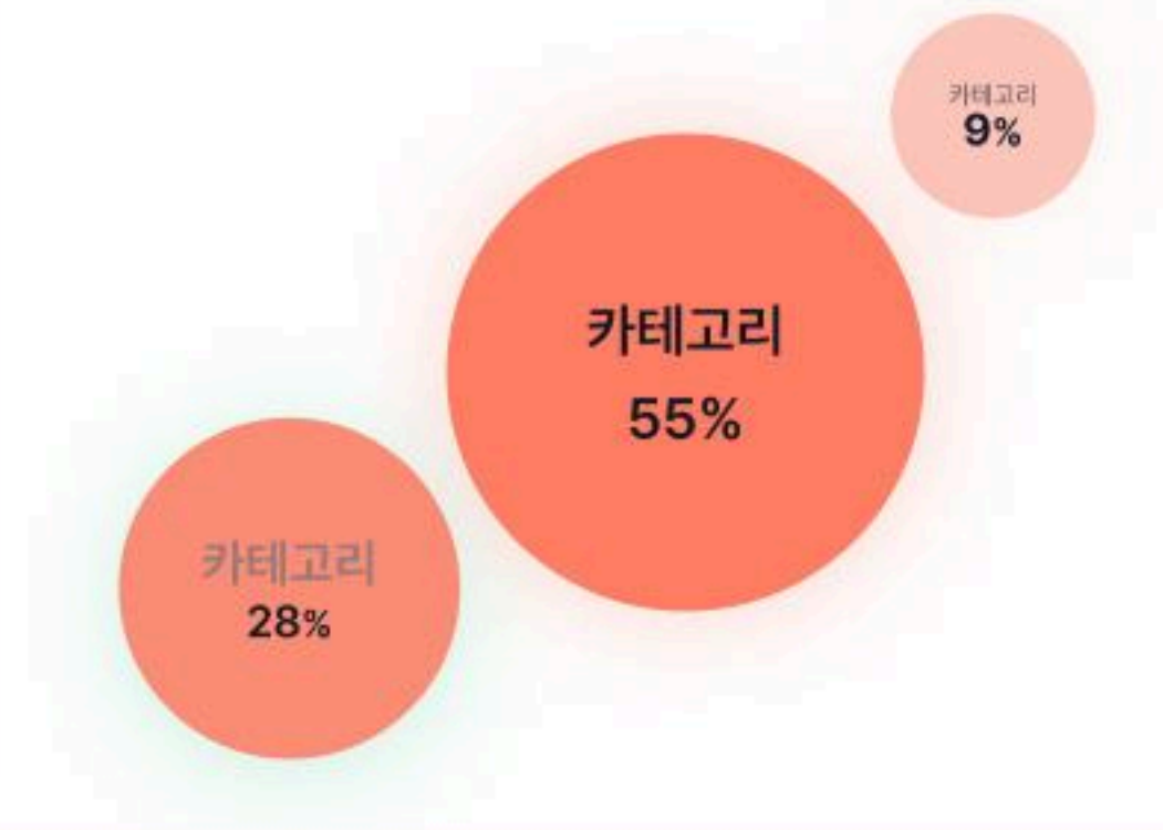
Bubble
